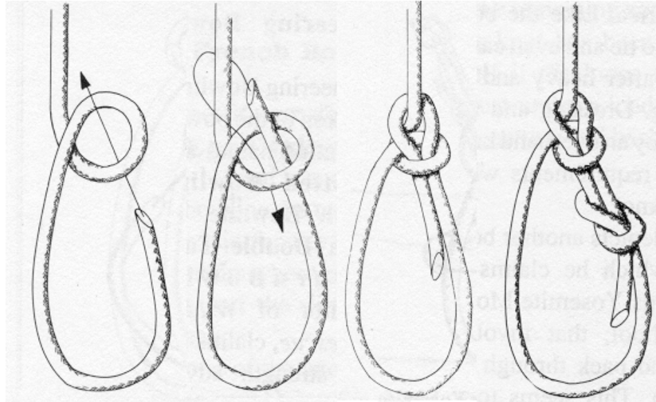
BOWLINE
