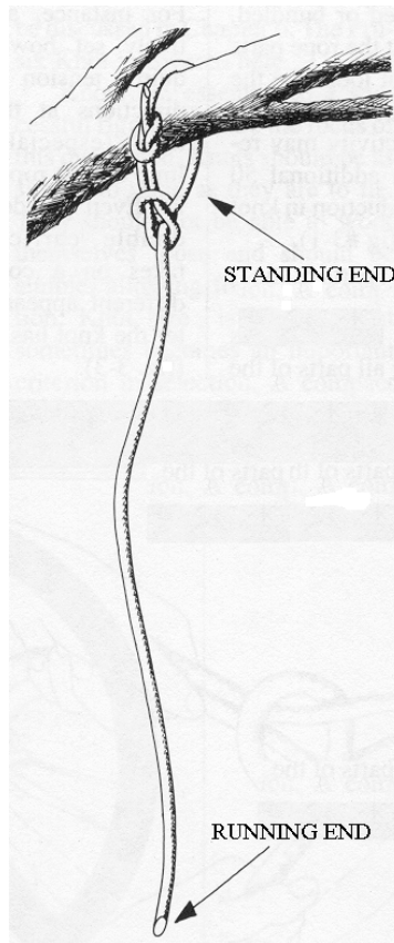
HALF HITCH
