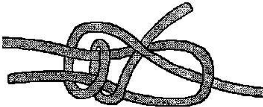
SHEET BEND
