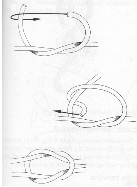
SQUARE KNOT
